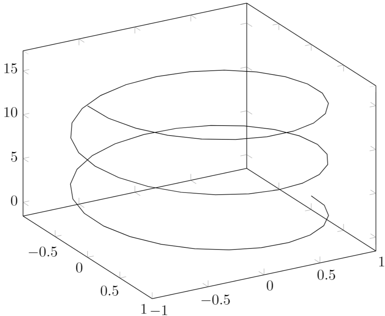
Figure 4: Some Plot 2
