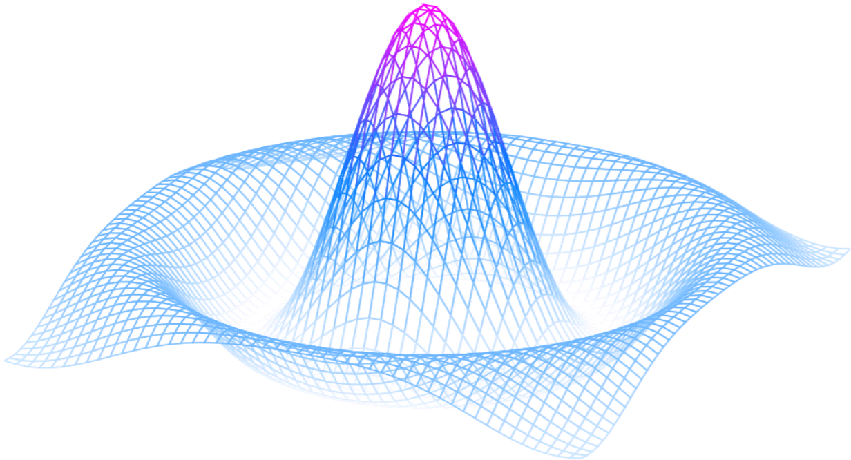
Figure 3: Some plot
